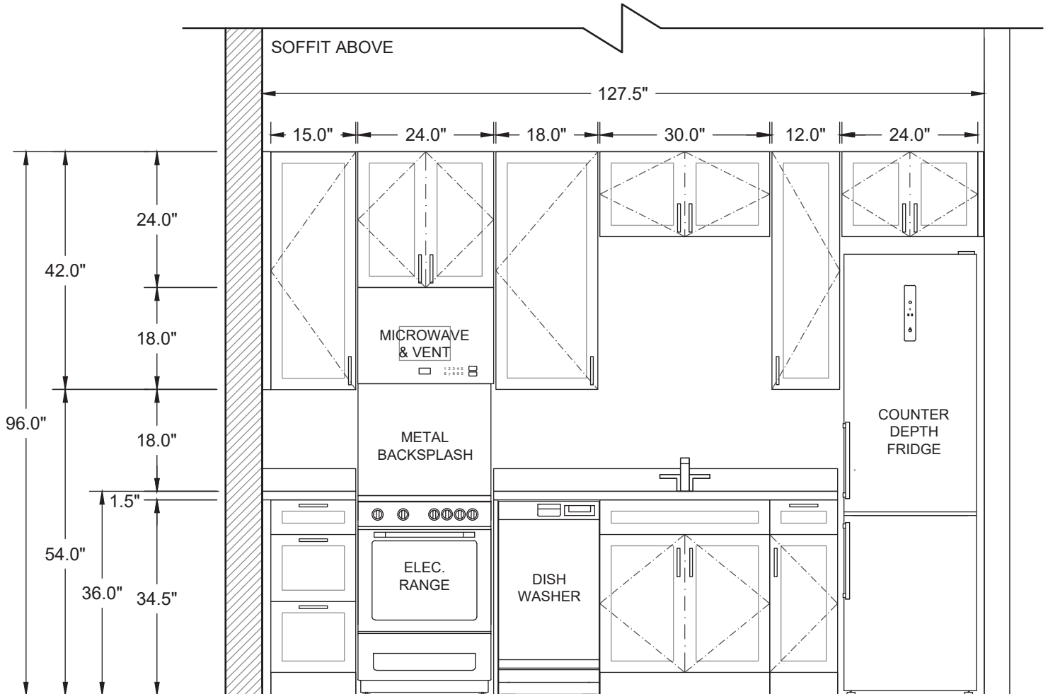
2 KITCHEN ELEVATION 2BD 2BATH UNIT
